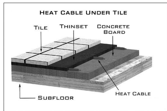
Figure 4: Heat cable installed under mosaic tile.
