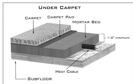
Figure 3: Example of heat cable installed in slab under carpet.
